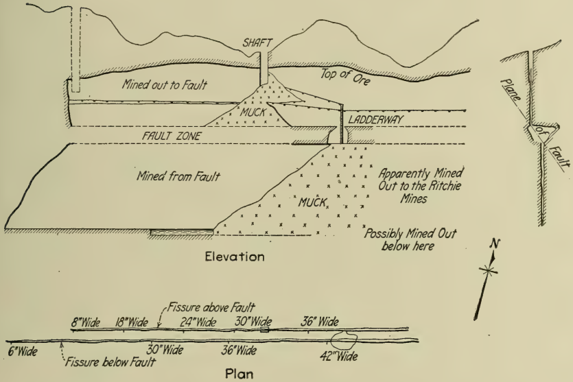
FIG. 51.—Sections through Grahamite Mine, Ritchie County, W. Va.
